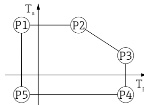
57 316L housing, hygiene; process temperature -60 to +150 °C ( -76 to +302 °F)
