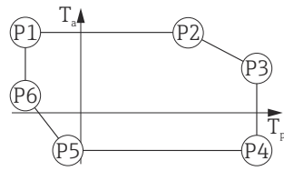
44 Aluminum housing, coated; process temperature -196 to +200 °C ( -320 to +392 °F)
