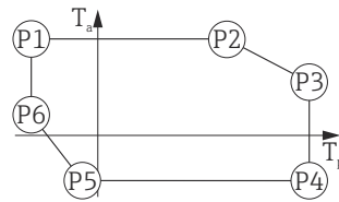
35 Plastic housing; process temperature -196 to +200 °C ( -320 to +392 °F)
