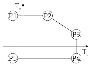
46 316L housing; process temperature -20 to +200 °C ( -4 to +392 °F)
