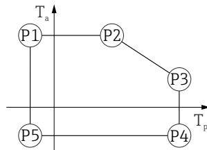
45 316L housing; process temperature -20 to +150 °C ( -4 to +302 °F)
