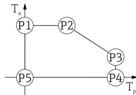
36 CSA C/US approval and plastic housing; process temperature 0 to +200 °C ( +32 to +392 °F)
