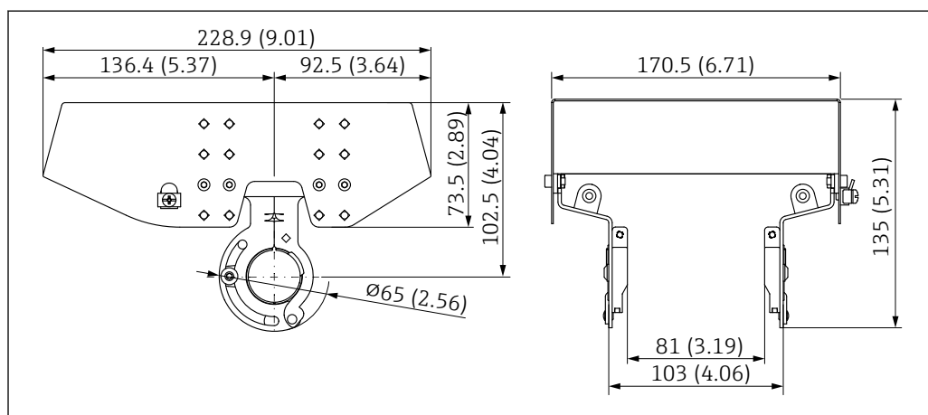
45 Protective cover for aluminum dual compartment housing. Unit of measurement mm (in)
