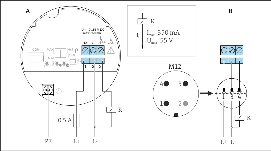
19 3-wire DC-PNP, electronic insert FEL62 A Connection wiring with terminals B Connection wiring with M12 plug in housing according to EN61131-2 standard
