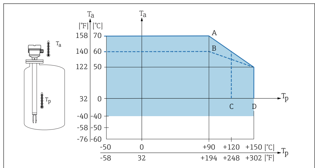
49 Permitted ambient temperature T_a at the housing as a function of the process temperature T_p in the vessel:
