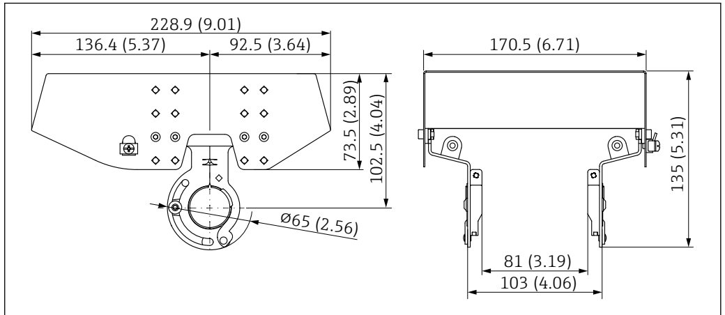
61 Protective cover for aluminum dual compartment housing. Unit of measurement mm (in)
