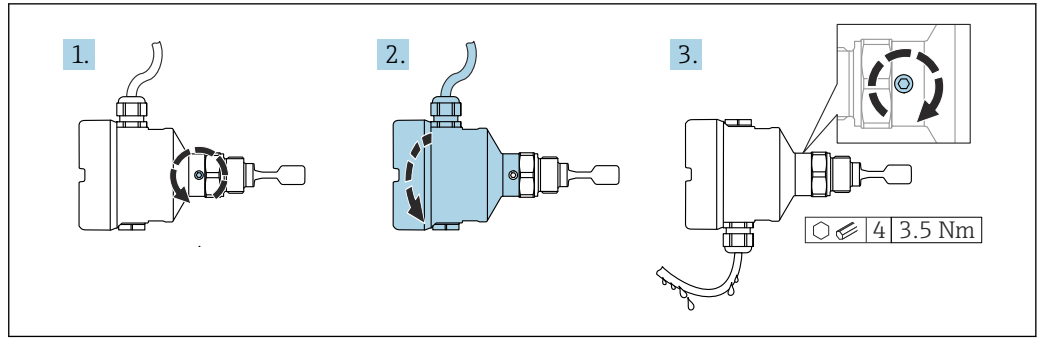
27 Housing with external locking screw and drip loop
