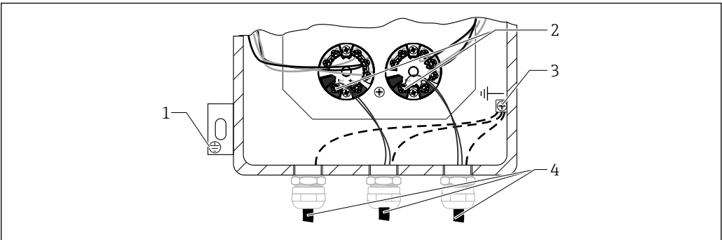
5 Connecting the signal cable and power supply to the installed transmitter
