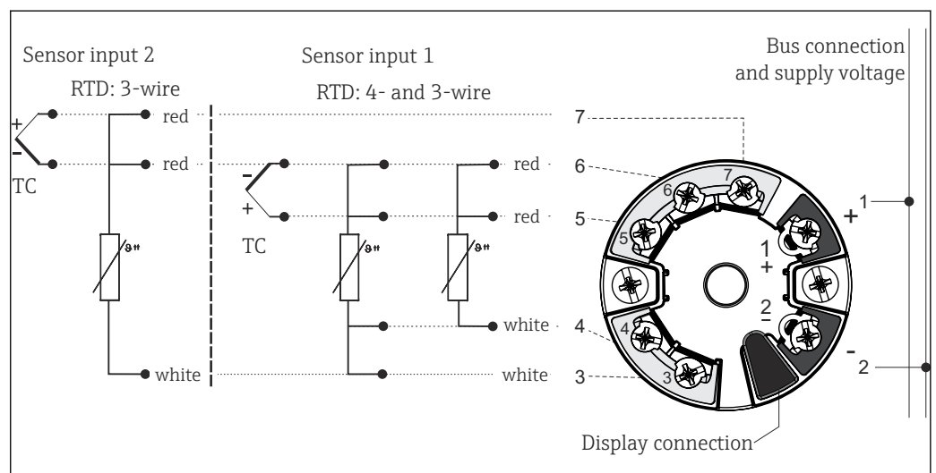
1 Wiring diagram of the dual sensor input head transmitters (TMT8x)
