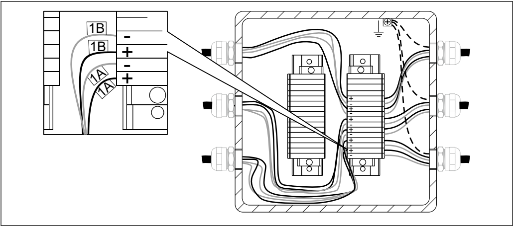
3 Direct wiring on the mounted terminal block. Example for the internal sensor wires marking with 2 x TC sensors in insert no. 1.
