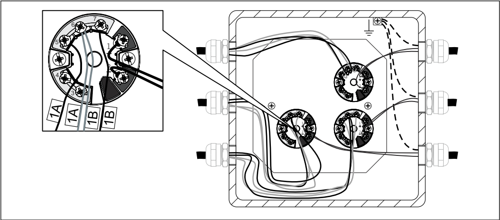
4 Mounted and wired head transmitter. Example for the internal sensor wires marking with 2 x TC
