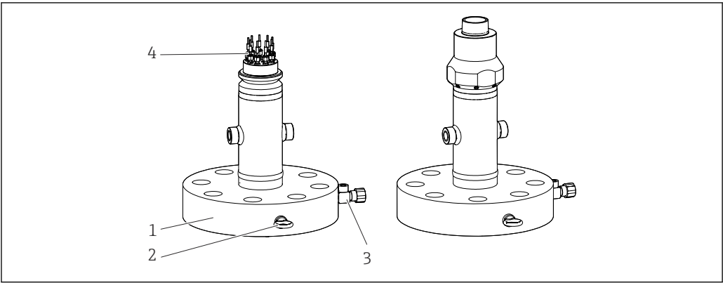
9 Flange as process connection
