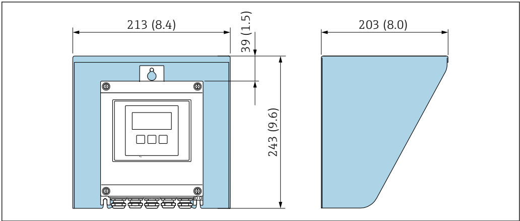
26 Weather protection cover; engineering unit mm (in)
