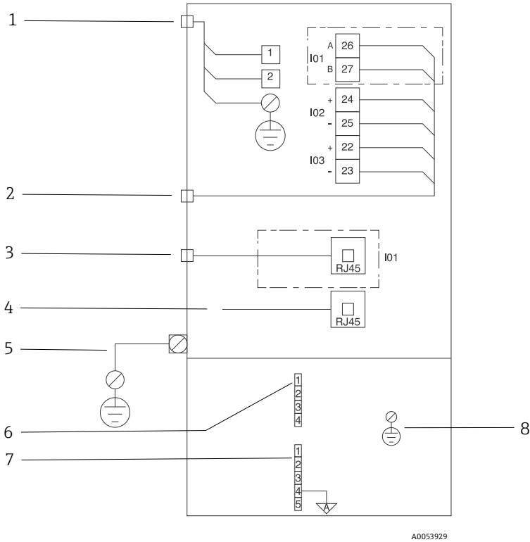
Figure 9. JT33 analyzer electrical connections
