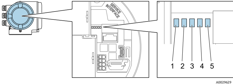
Figure 30. LED diagnostic indicators
