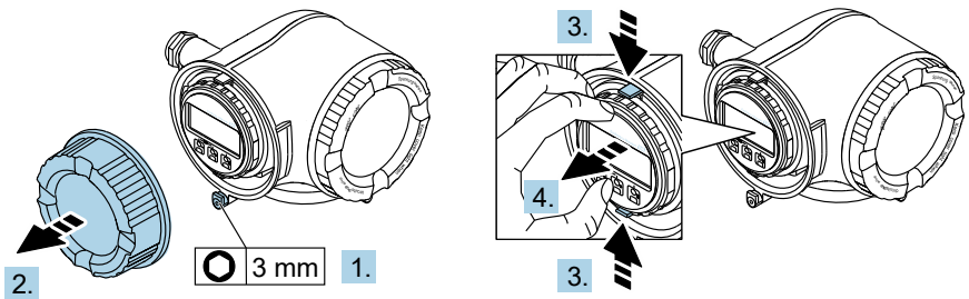
Figure 16. Removing the display module holder
