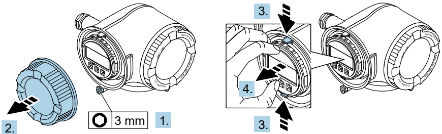
Figure 12. Removing the display module holder
