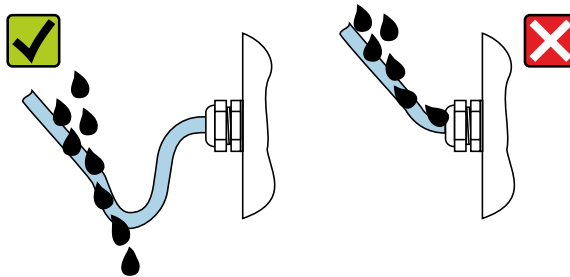
Figure 23. Ensuring IP66 degree of protection
