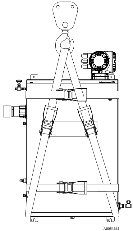
Figure 2. JT33 analyzer with ratchet straps for lifting and moving
