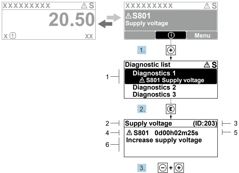
Figure 32. Message for remedial measures
