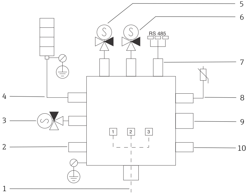
Figure 10. MAC enclosure designed instrument/sensor locations
