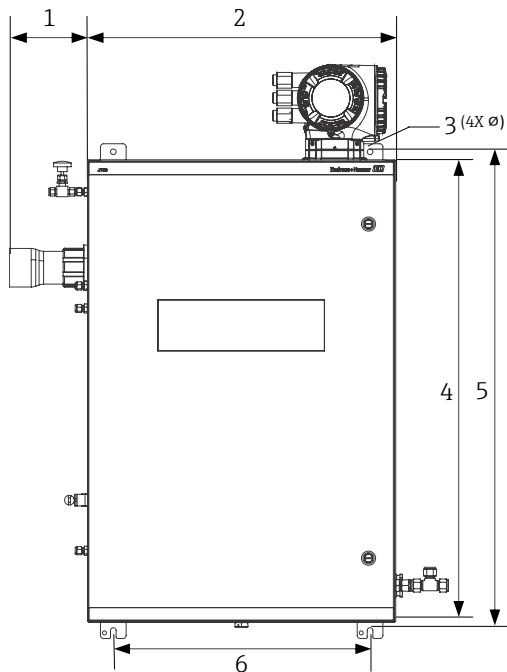
Figure 4. Mounting dimensions: Front view
