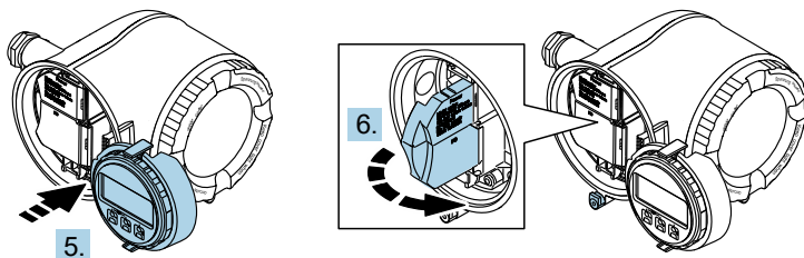
Figure 17. Opening the terminal cover
