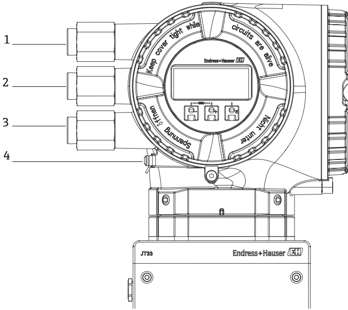
Figure 11. Threaded entries
