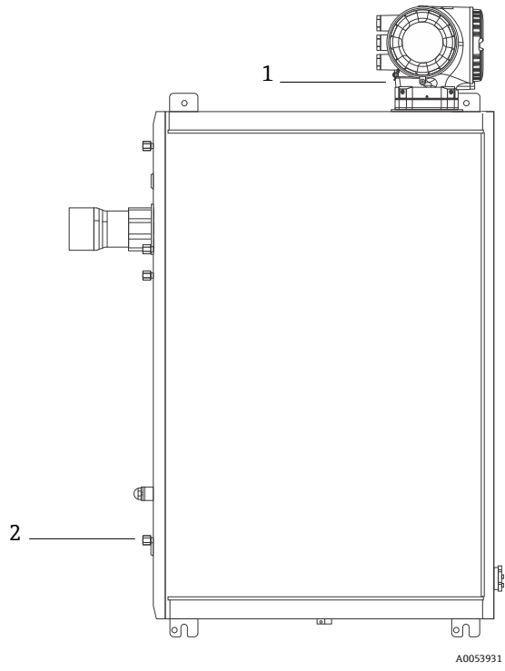
Figure 8. Ground connections
