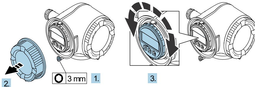
Figure 7. Turning the display module
