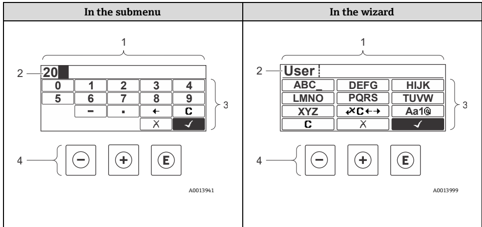
Figure 28. Editing view in the submenu and in the wizard
