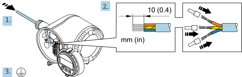
Figure 19. Feeding wiring and connecting the protective ground
