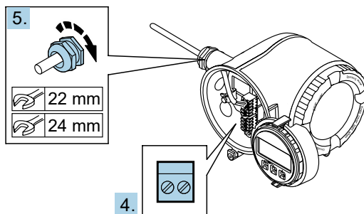
Figure 15. Connecting the cables and tightening glands
