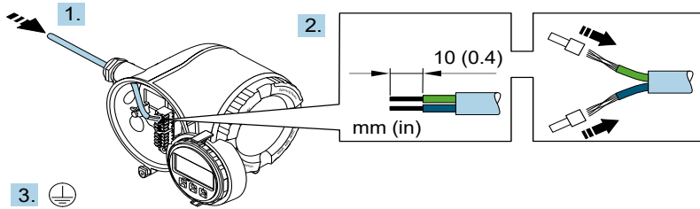
Figure 14. Feeding wiring and connecting the protective ground
