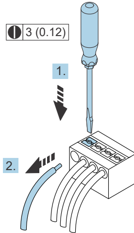
Figure 20. Removing a cable. Engineering unit: mm (in)
