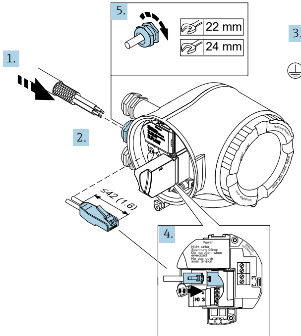
Figure 18. Connecting the RJ45 cable
