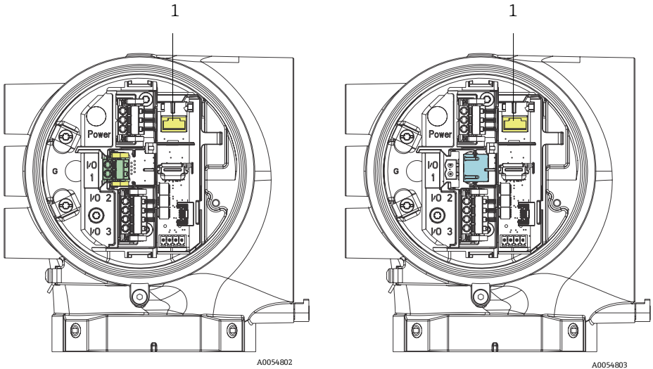
Figure 21. Service interface CDI-RJ45 (1) connections for I/O1 with Modbus RTU/RS485/2-wire (left) and Modbus TCP/Ethernet/RJ45 (right)
