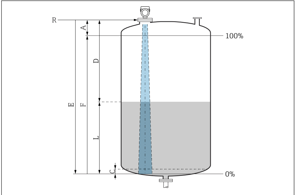
4 Configuration parameters for level measurement in liquids
