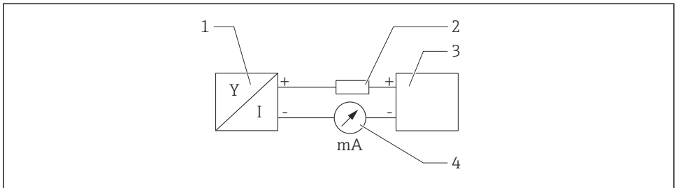
2 Block diagram of HART connection
