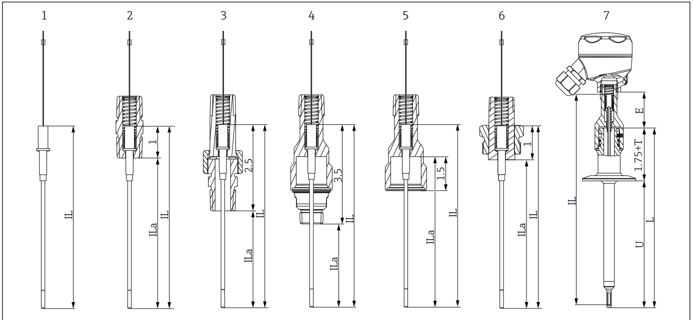
3 Design of the iTHERM TS212
