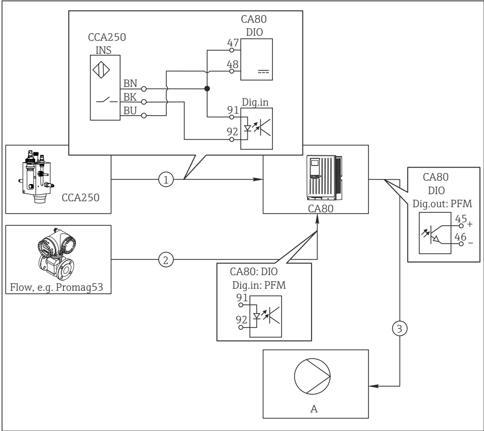
62 Example of chlorine control with feedforward control
