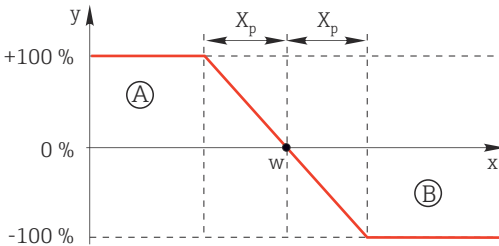
74 Red: overlap between the curves of the two 1-sided controllers.
