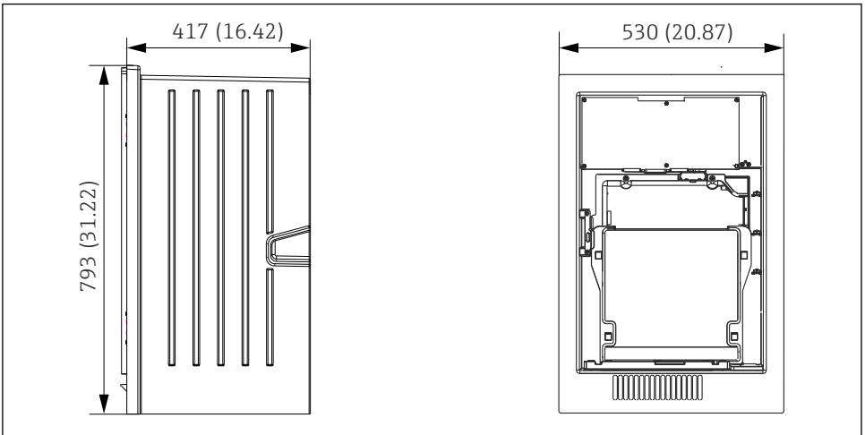
13 Liquiline System CA80 open version, dimensions in mm (in)
