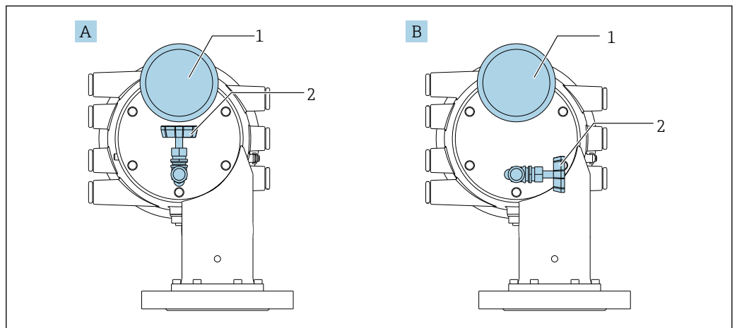
29 Mounting position of relief valve and pressure gauge
