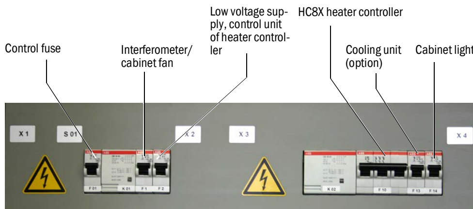
Fig. 14 Fuses, system cabinet
