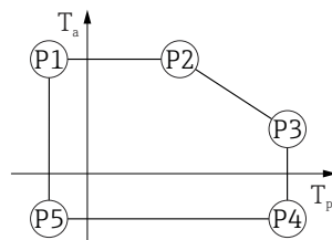
35 Aluminum housing, coated; process temperature -10 to +200 °C (+14 to +392 °F)
