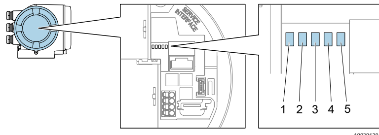
Figure 65. Indicateurs de diagnostic LED
