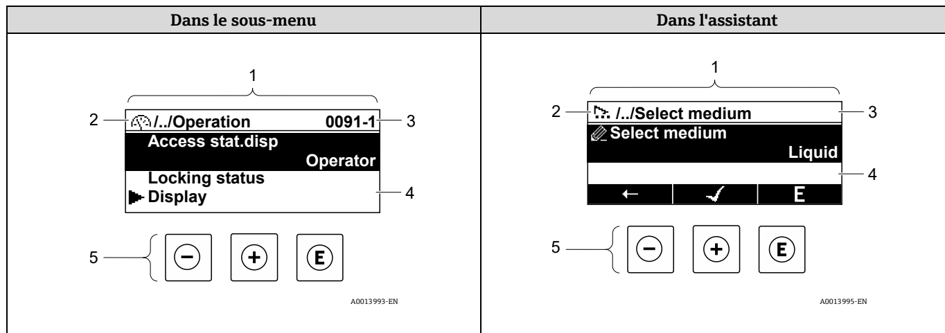
Figure 43. Vue navigation
