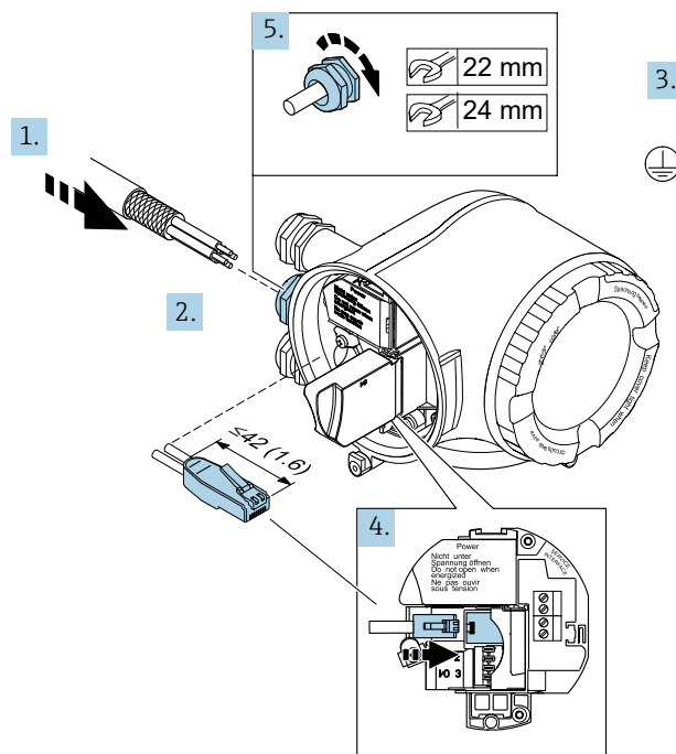
Figure 20. Raccordement du câble RJ45
