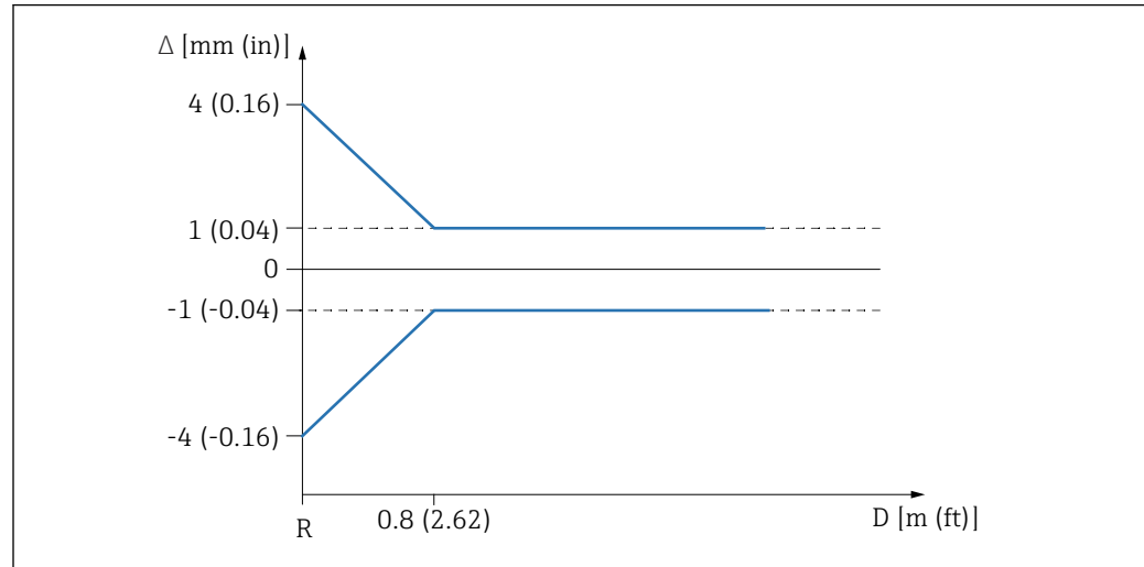
9 Maximum measured error in near-range applications
