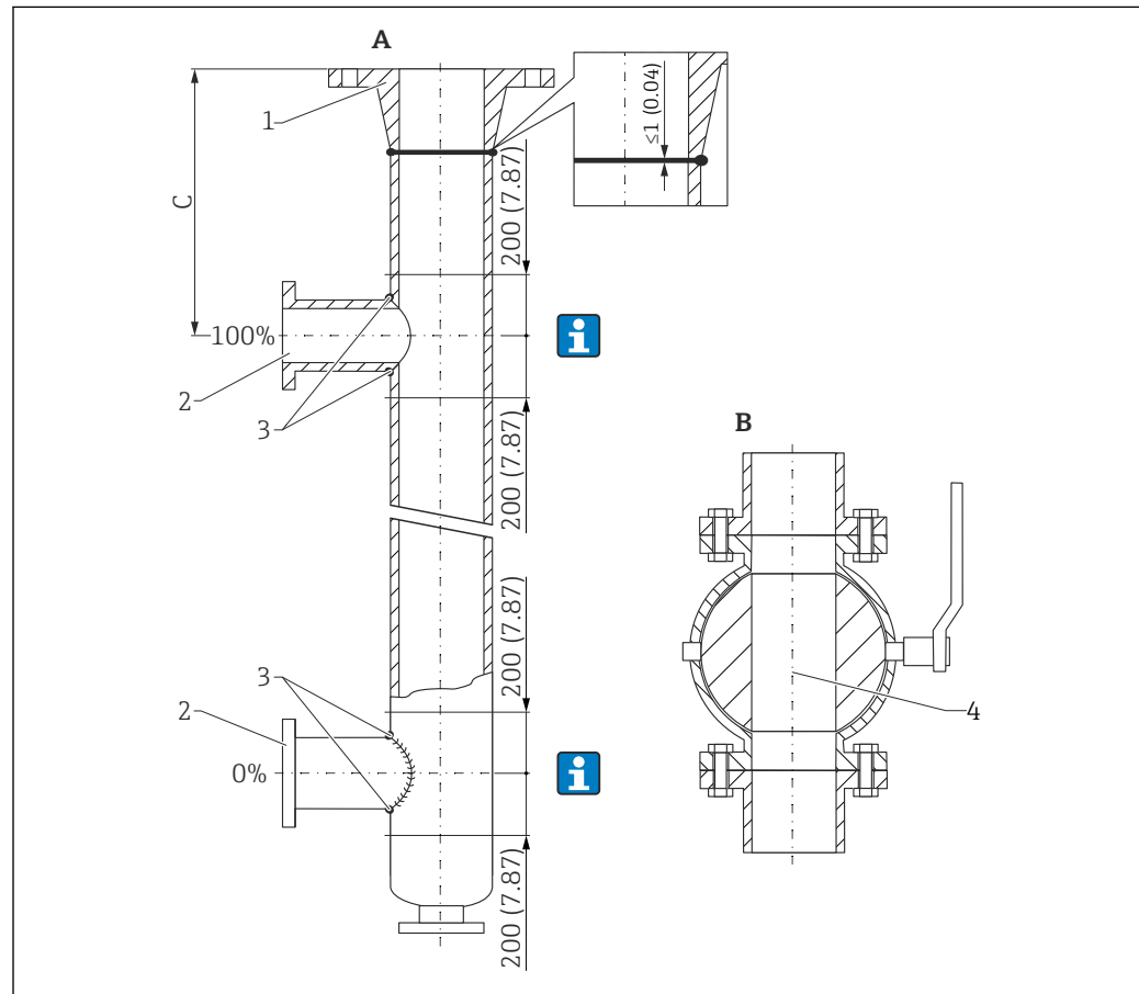
14 Example of bypass design. Unit of measurement mm (in)
