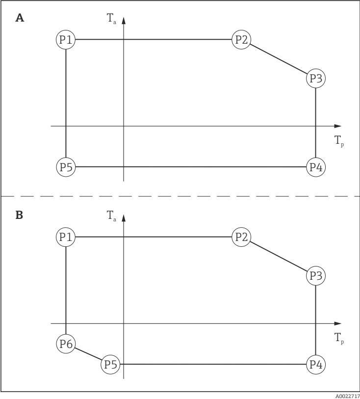
Example diagrams of possible deratings
