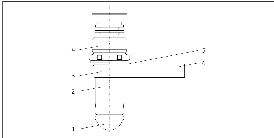
45 Material; antena tipo drip-off 50 mm (2 in)
