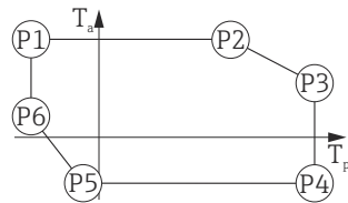
▣ 45 铝外壳，带涂层；过程温度：-196 ... +200 °C (-320 ... +392 °F)
