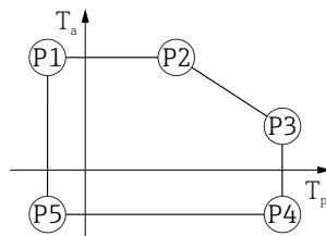
☑ 13 塑料外壳; 过程温度范围: -20 \dots +200 \text{ }^\circ\text{C} ( -4 \dots +392 \text{ }^\circ\text{F} )
