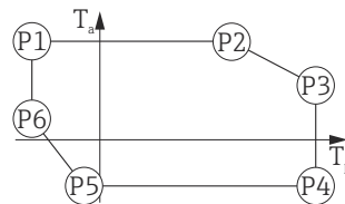
29 塑料外壳; 过程温度: -196 \dots +200 \text{ }^\circ\text{C} ( -320 \dots +392 \text{ }^\circ\text{F} )
