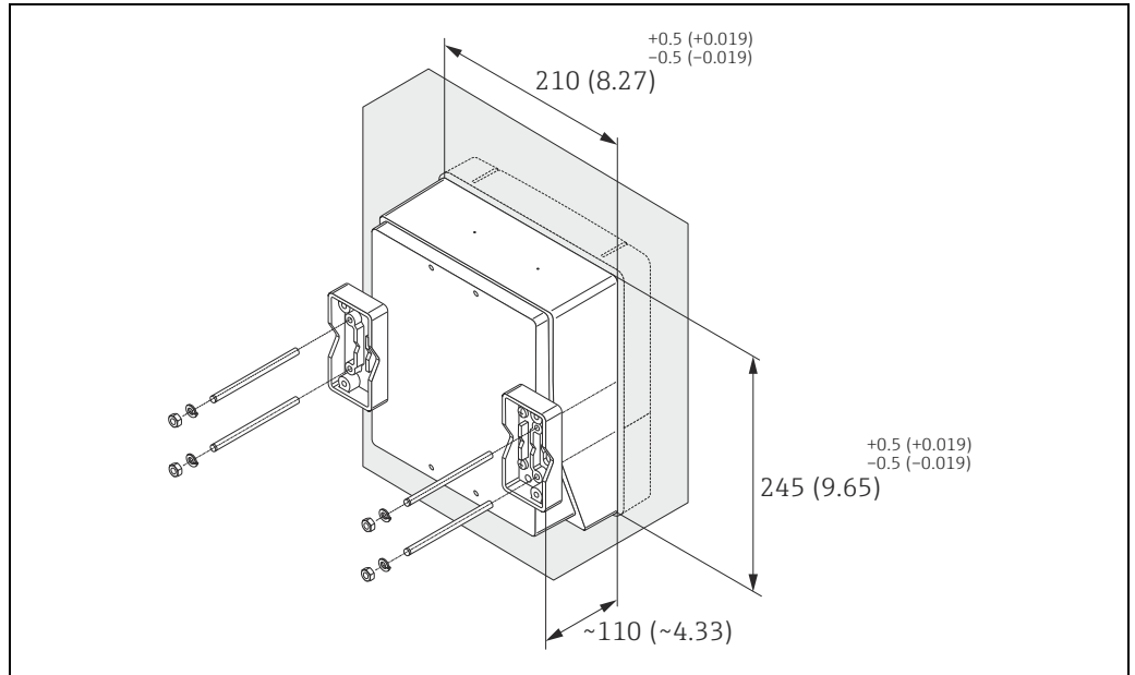
Panel-mounted installation. Engineering unit mm (in)
