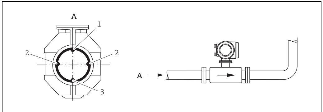
Horizontal orientation
