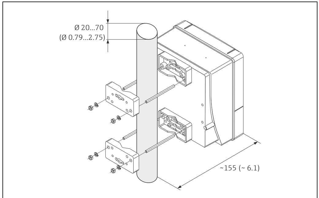
Pipe mounting. Engineering unit mm (in)
