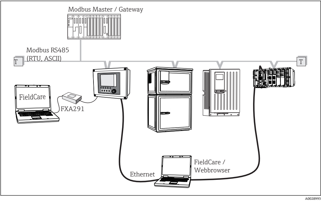
13 Modbus RS485
