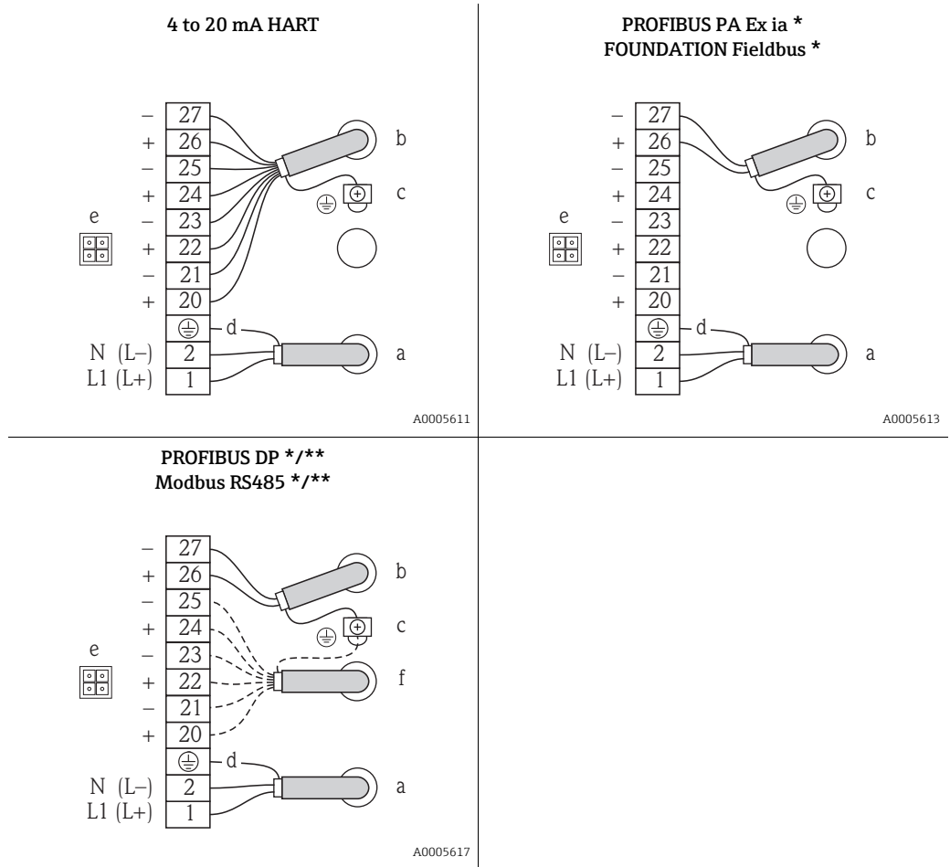
Fig. 10: Electrical connections
