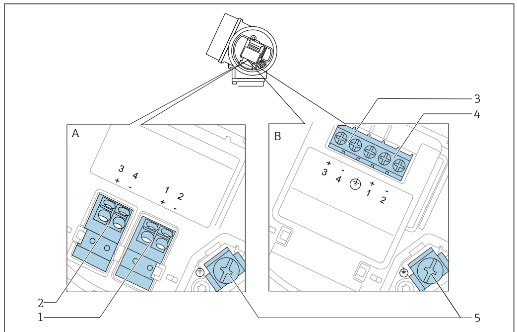
13 接线端子分配: PROFIBUS PA / FOUNDATION Fieldbus
