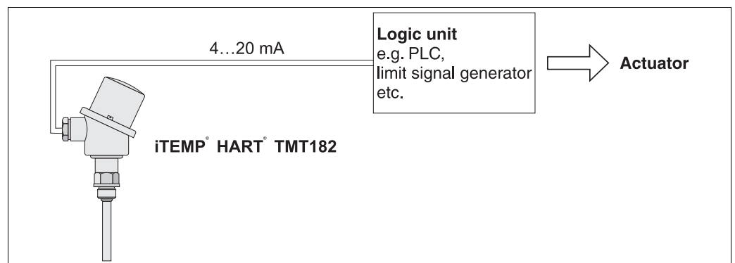
Fig. 2: safety function (e.g. for limit temperature monitoring) with TMT 182 as sub-system
