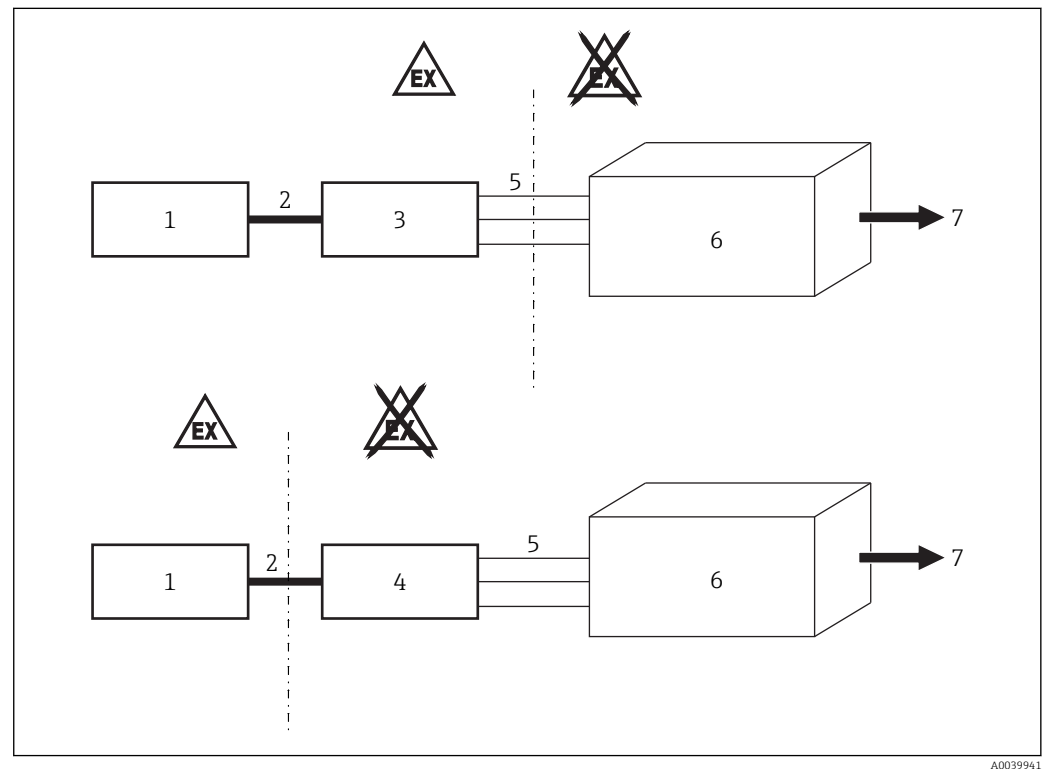
4 System diagram
