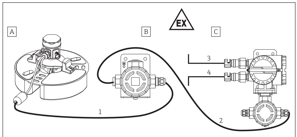
3 System design 3 (TIS qualification: TC18324 (NAR300) / TC18327 (FTL) / TC18325 (NRR261))
