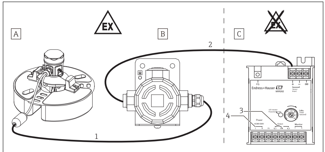
2 System design 2
