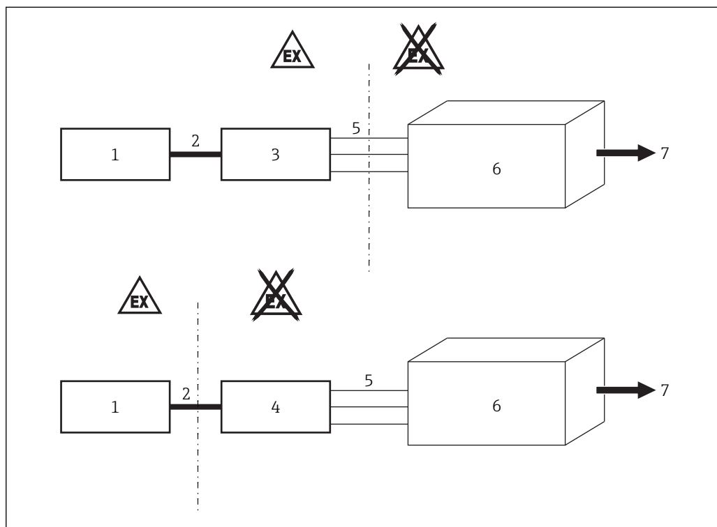
4 System diagram
