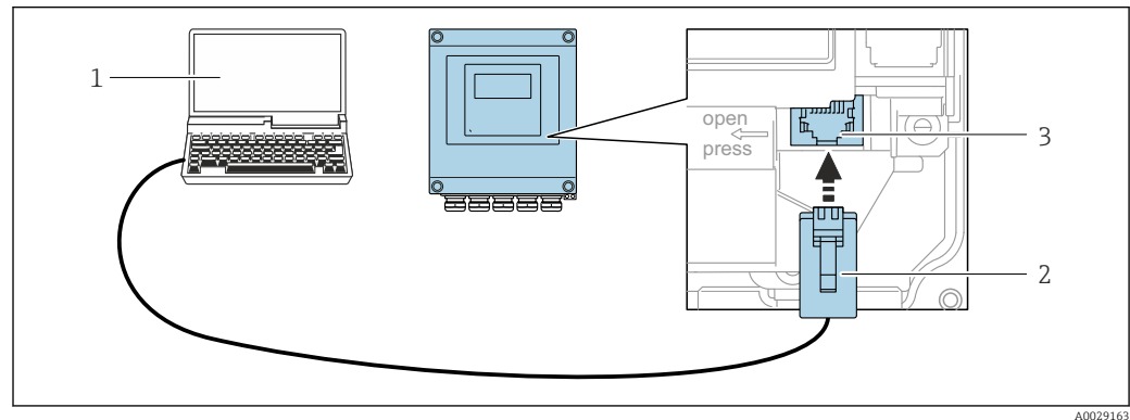
79 Connection via service interface (CDI-RJ45)
