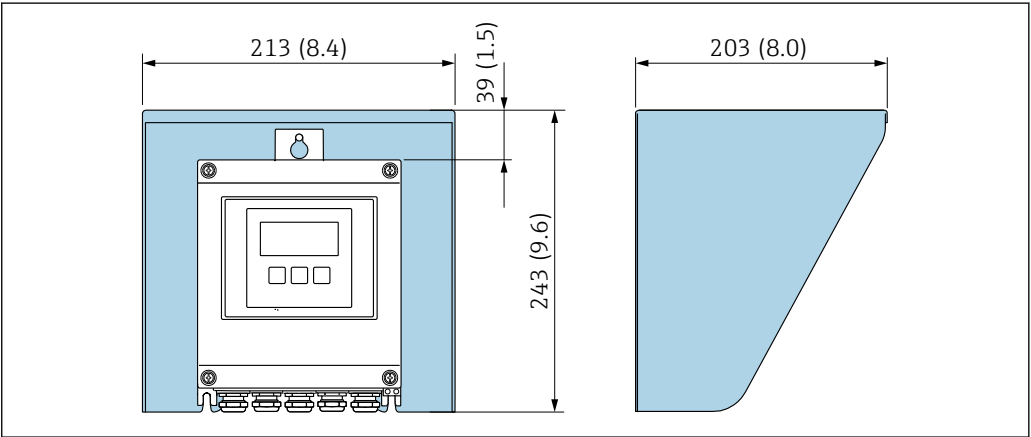
60 Weather protection cover for Proline 500 – digital
