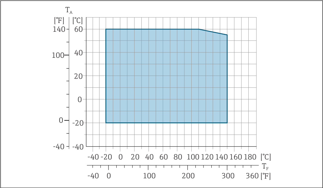
32 Promag 500 T_A Ambient temperature range T_F Fluid temperature
