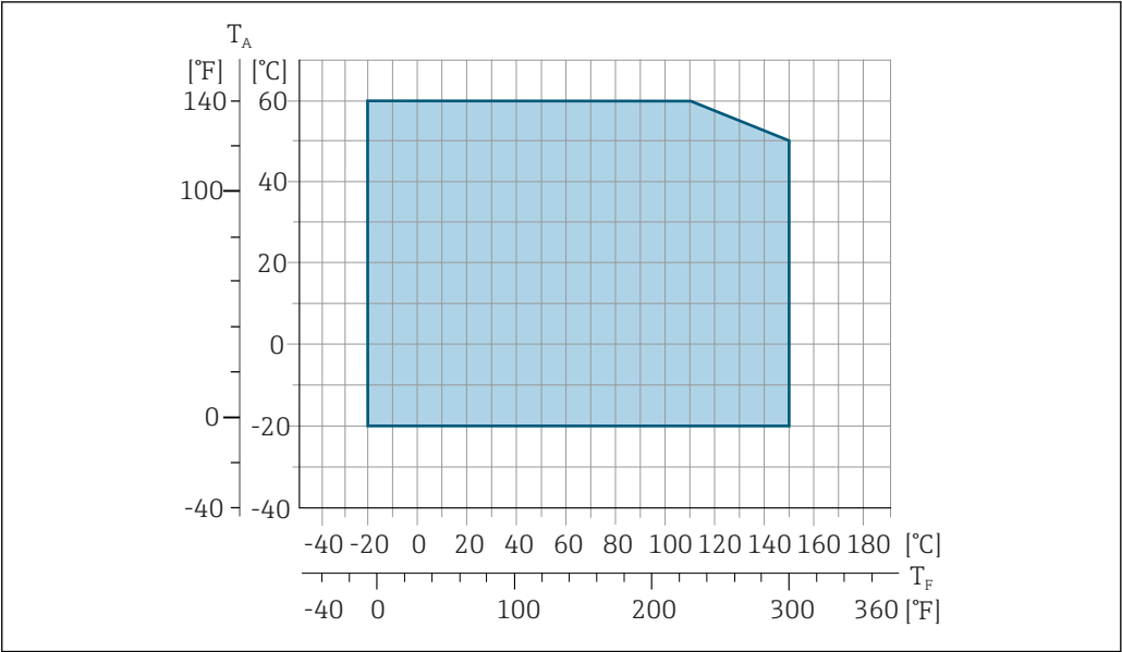
31 Promag 500 – digital T_A Ambient temperature range T_F Fluid temperature
