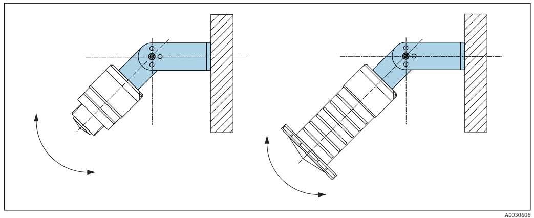
18 Installation with mounting bracket, adjustable
