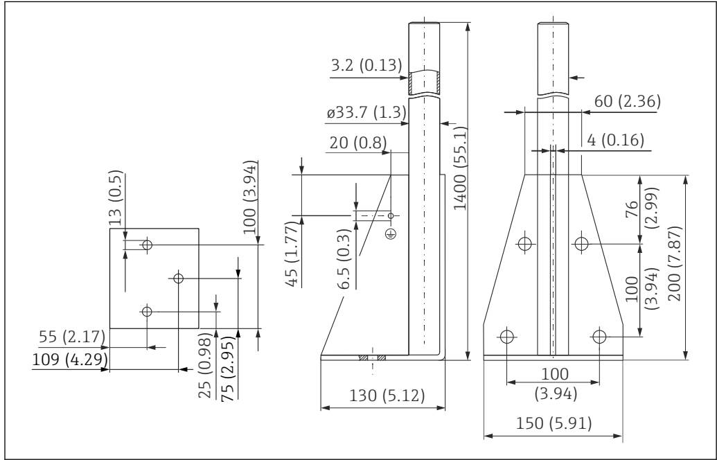
18 Dimensions. Unit of measurement mm (in)
