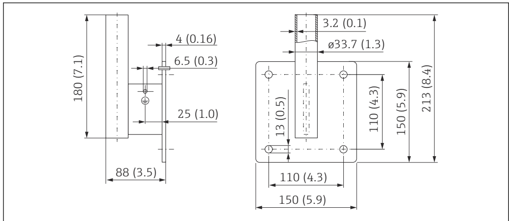
19 Dimensions of the wall bracket. Unit of measurement mm (in)
