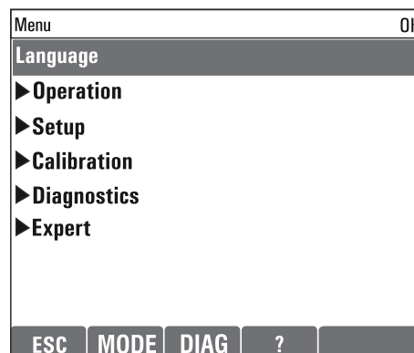
17 Plain-text menu
