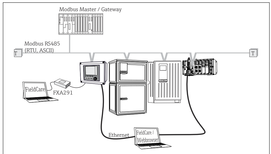
19 Modbus RS485
