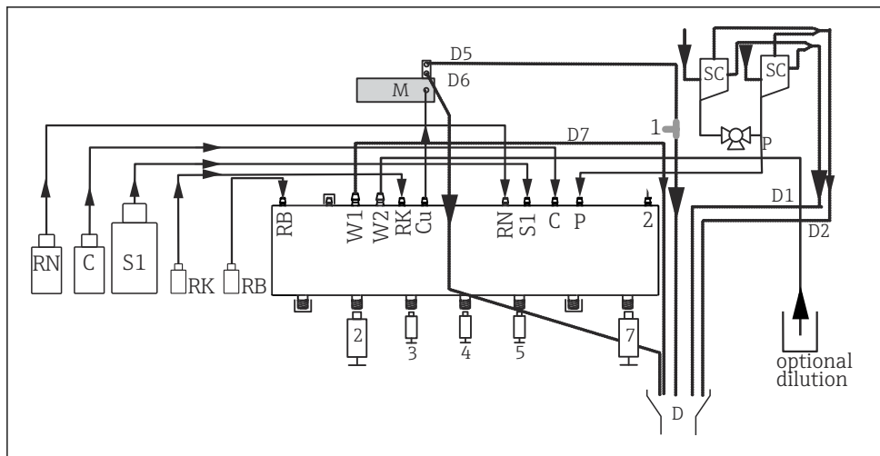
24 Liquiline System CA80AL, two-channel device
