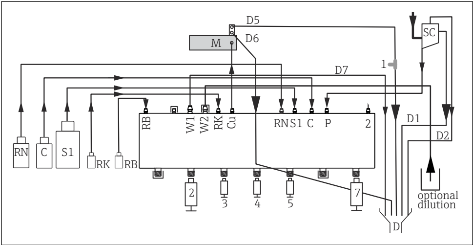
23 Liquiline System CA80AL, single-channel device
