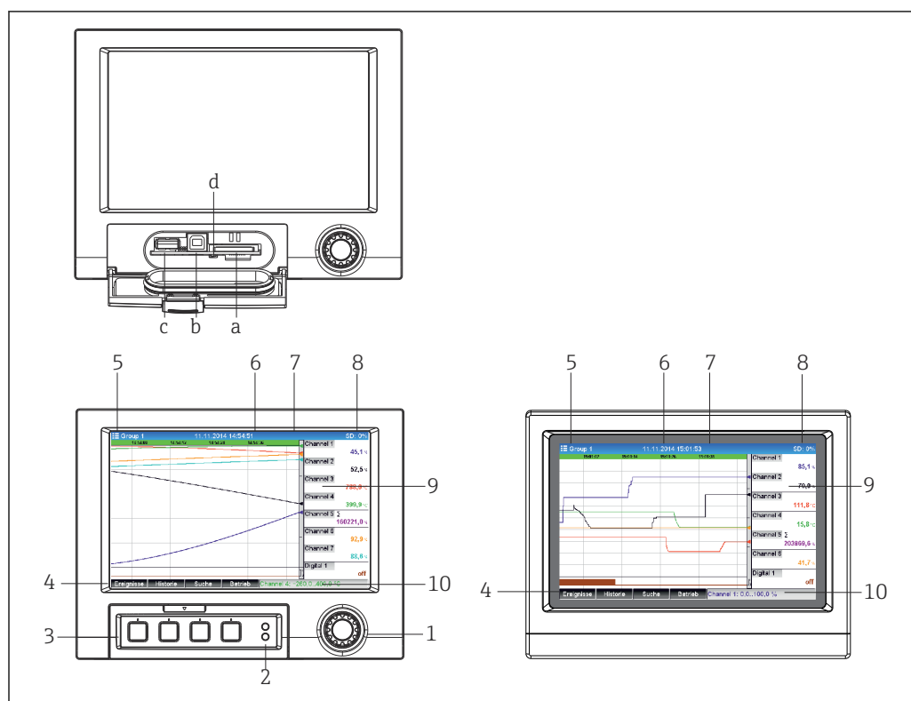
6 Device front (left: version with navigator and front interfaces; right: version with stainless steel front and touchscreen)
