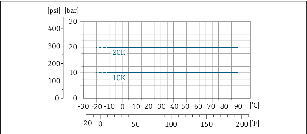
23 Matériau du raccord process : inox (-20 °C (-4 °F)) ; acier au carbone (-10 °C (14 °F))
