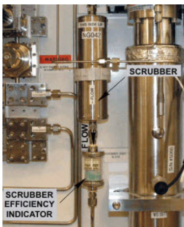
Figure 5-5 Scrubber and scrubber efficiency indicator
