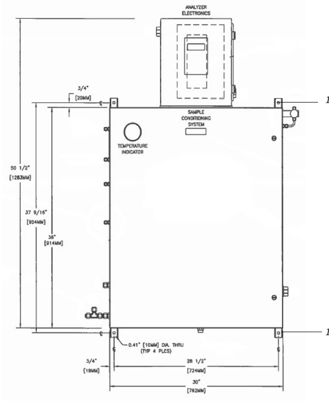
Figure 3-1 Lifting points for the SS2100 H 2 S analyzer
