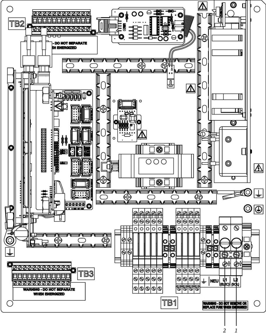
Figure 5-1 H 2 S analyzer electronics control board (AC) showing fuses
