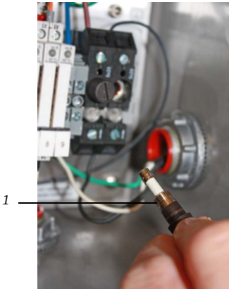
Figure 5-4 Replacing fuse
