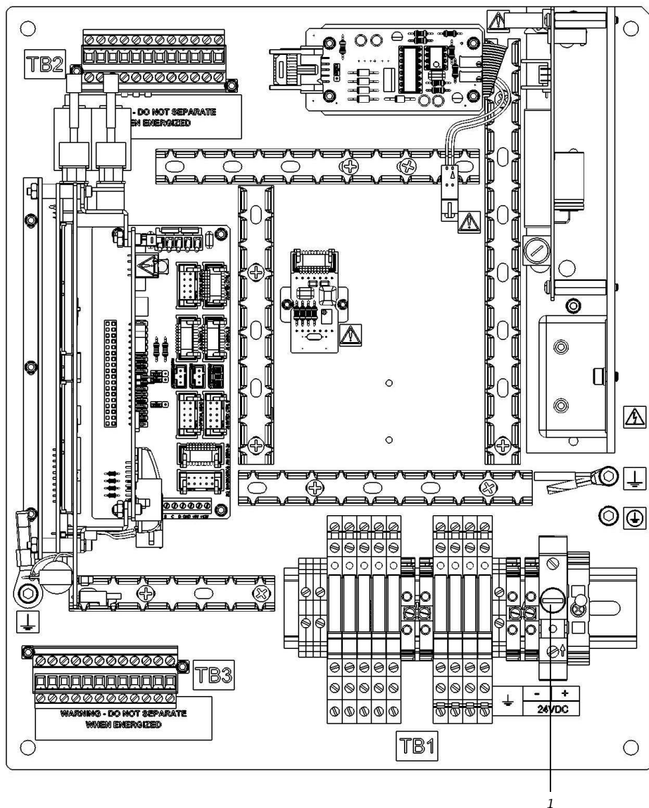
Figure 5-2 H 2 S analyzer electronics control board (DC) showing fuses
