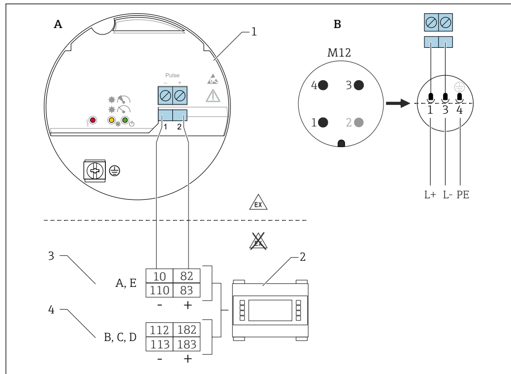
16 Connection diagram: Connecting the FEL60D electronic insert to the Density Computer FML621
