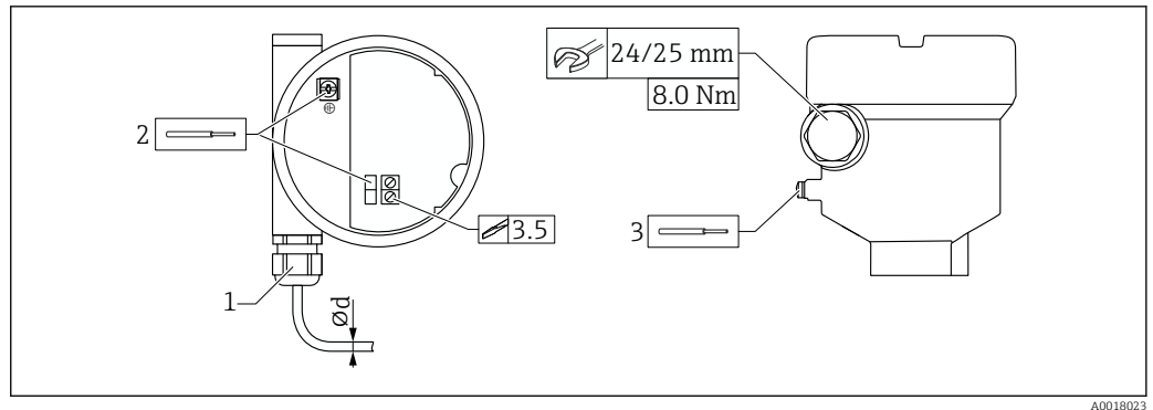
18 Example of coupling with cable entry, electronic insert with terminals
