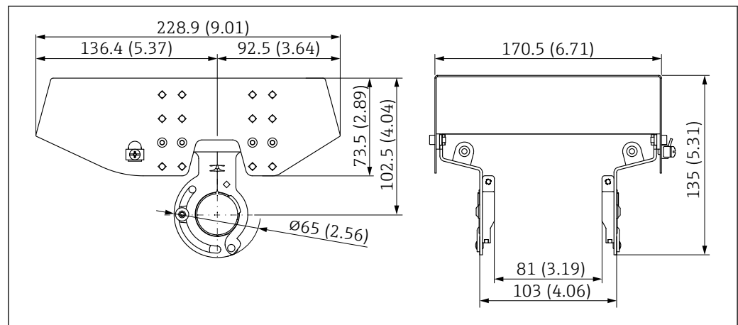
20 Weather protection cover for dual compartment housing, aluminum. Unit of measurement mm (in)
