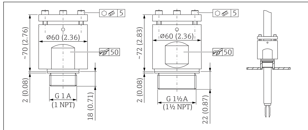
23 High pressure sliding sleeves. Unit of measurement mm (in)
