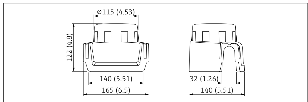
21 Weather protection cover for single compartment housing made of aluminum or 316L, cast. Unit of measurement mm (in)
