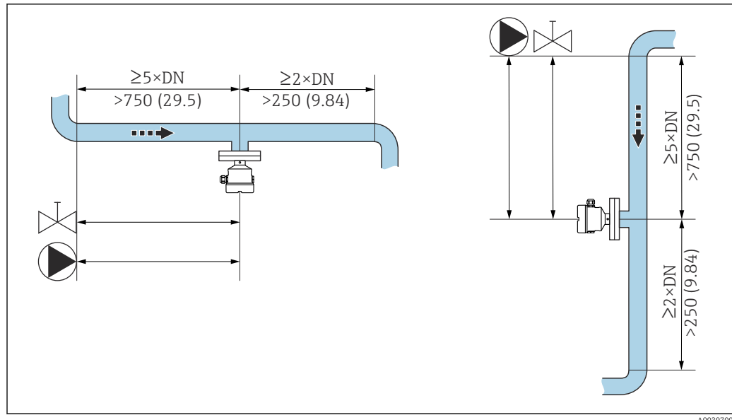
6 Installing the inlet run. Unit of measurement mm (in)
