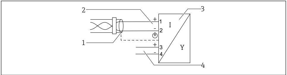
3 Kopplingsdiagram PROFIBUS PA/FOUNDATION Fieldbus
