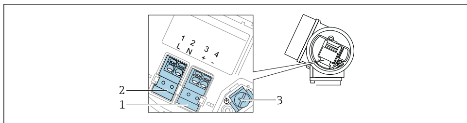
12 Klembezetting, 4-draads: 4 ... 20 mA HART (90 ... 253 V AC )
