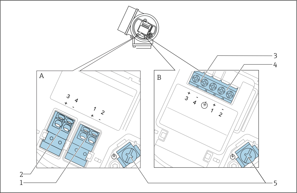
17 接线端子分配: 两线制; 4...20 mA HART, 4...20 mA
