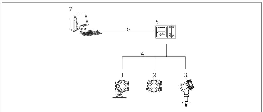
22 Remote operation of Tank Gauging devices
