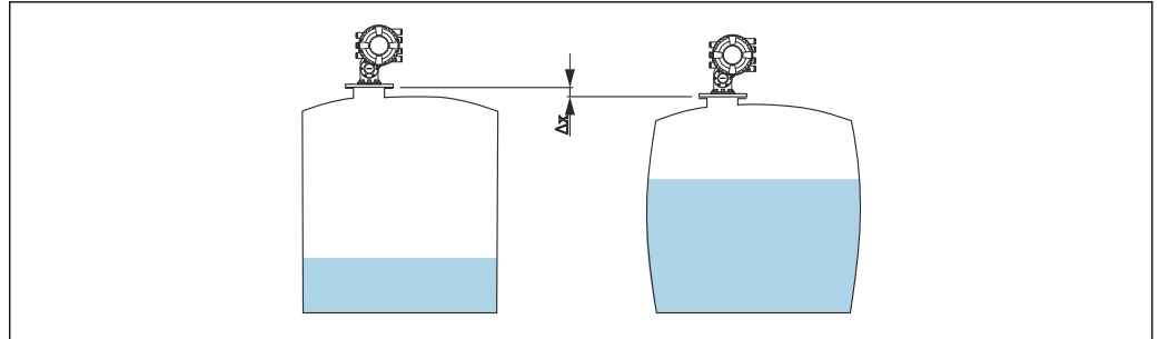
24 Movement \Delta x of the tank reference height due to the bulging of the tank shell caused by hydrostatic pressure
