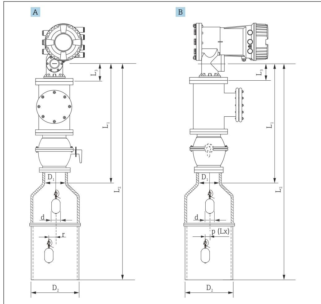
14 Mounting with concentric stilling well
