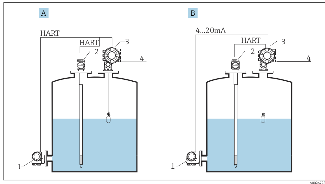
2 Measuring system for NMS80/NMS81
