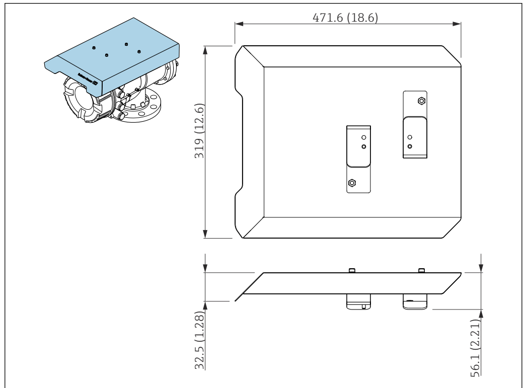
23 Weather protection cover; dimensions: mm (in)
