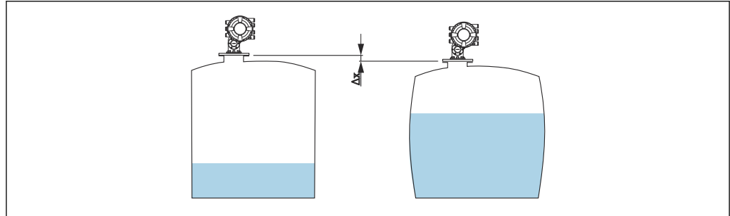
22 Movement \Delta x of the tank reference height due to the bulging of the tank shell caused by hydrostatic pressure
