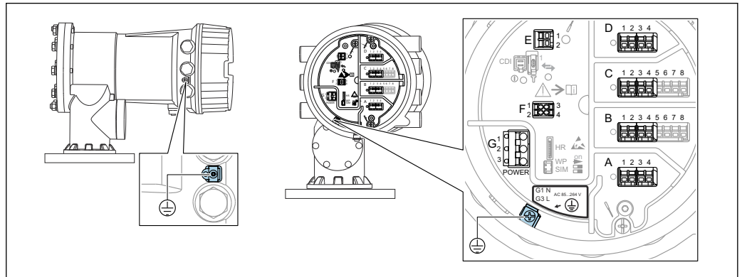
11 Terminal compartment (typical example) and ground terminals
