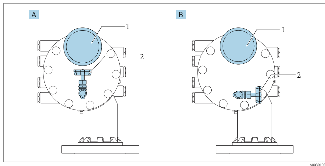
24 Mounting position of relief valve and pressure gauge
