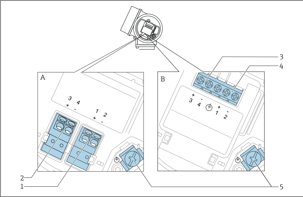
9 接线端子分配: PROFIBUS PA / FOUNDATION Fieldbus
