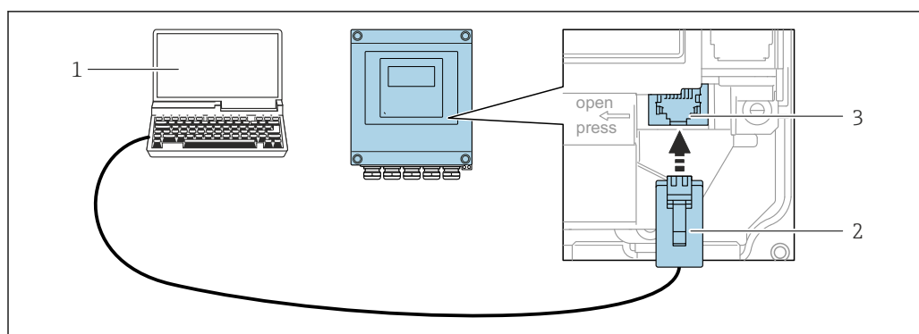
63 Raccordement via interface service (CDI-RJ45)
