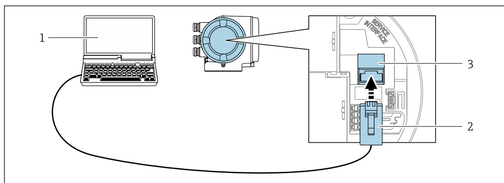
64 Raccordement via interface service (CDI-RJ45)
