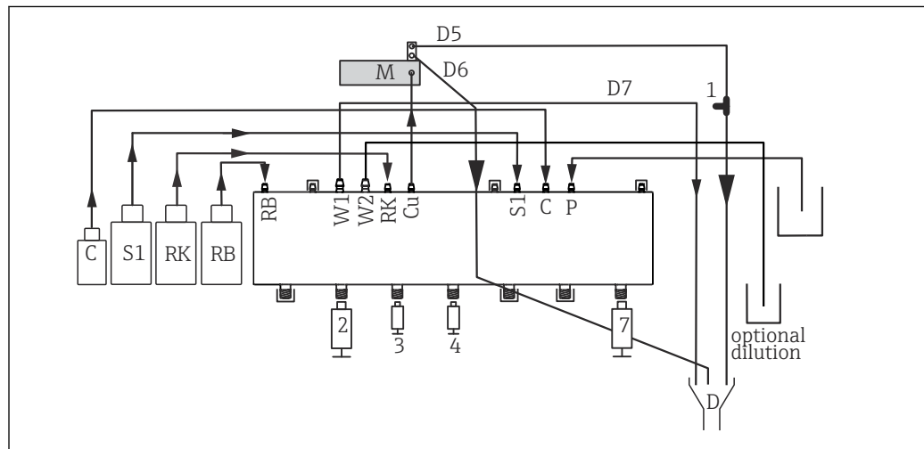
66 Liquiline System CA80CR, Selbstansauger
