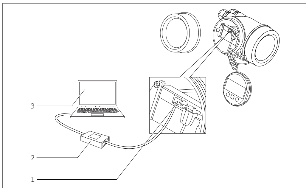
46 DeviceCare/FieldCare via interface service (CDI)
