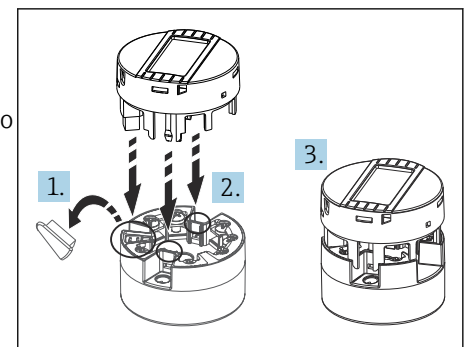
16 Instalar o display no transmissor
