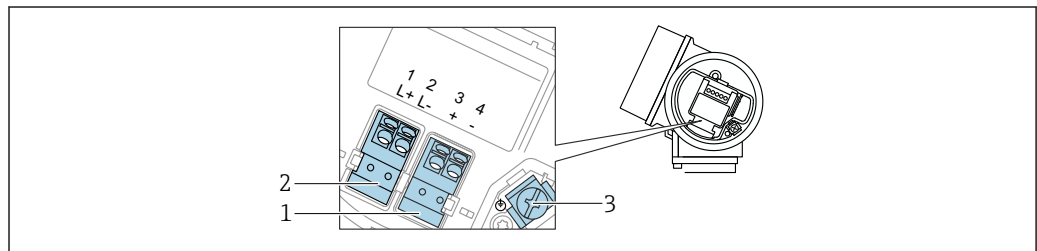
11 Terminal assignment, 4-wire: 4 to 20 mA HART (10.4 to 48 V DC )
