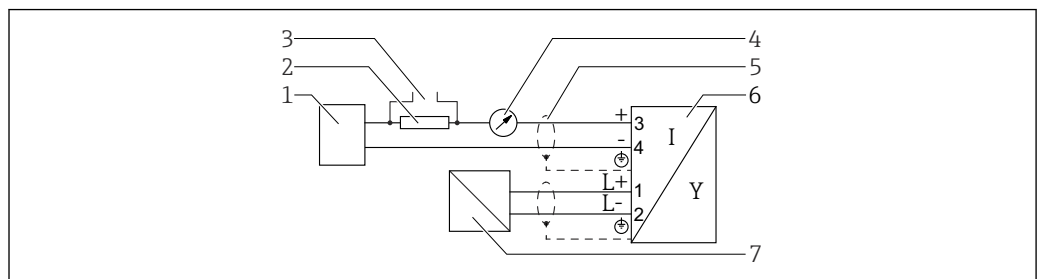
12 Block diagram, 4-wire: 4 to 20 mA HART (10.4 to 48 V DC )
