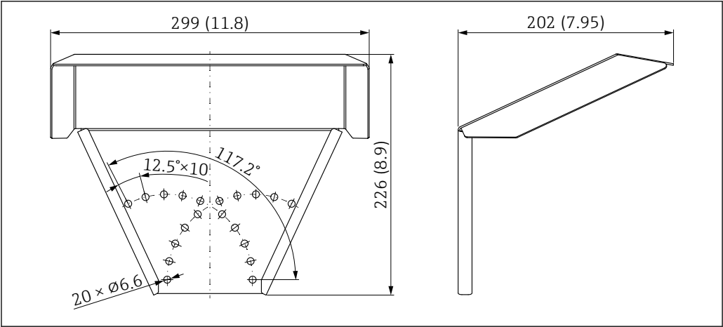
48 Dimensions. Unit of measurement mm (in)
