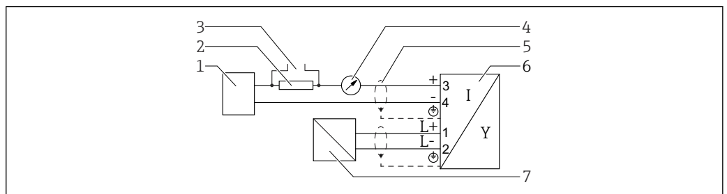
13 Blockdiagramm 4-Draht: 4 ... 20 mA HART (10,4 ... 48 V DC )
