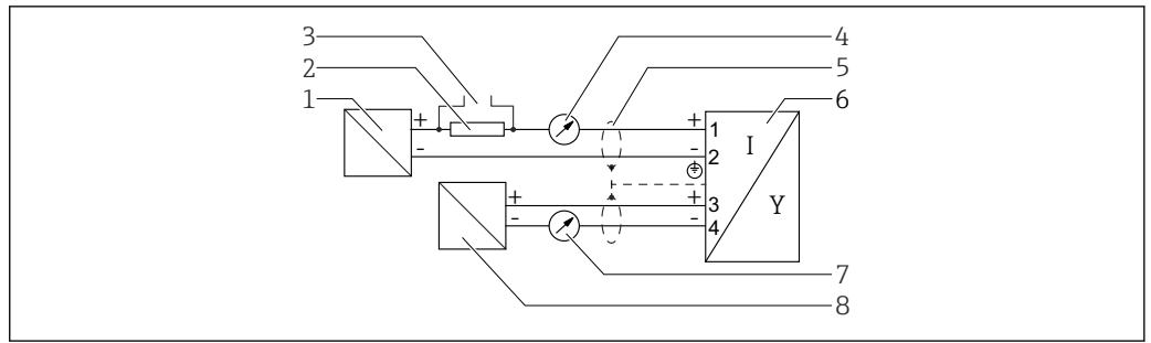
11 Blockdiagramm 2-Draht: 4 ... 20 mA HART, 4 ... 20 mA
