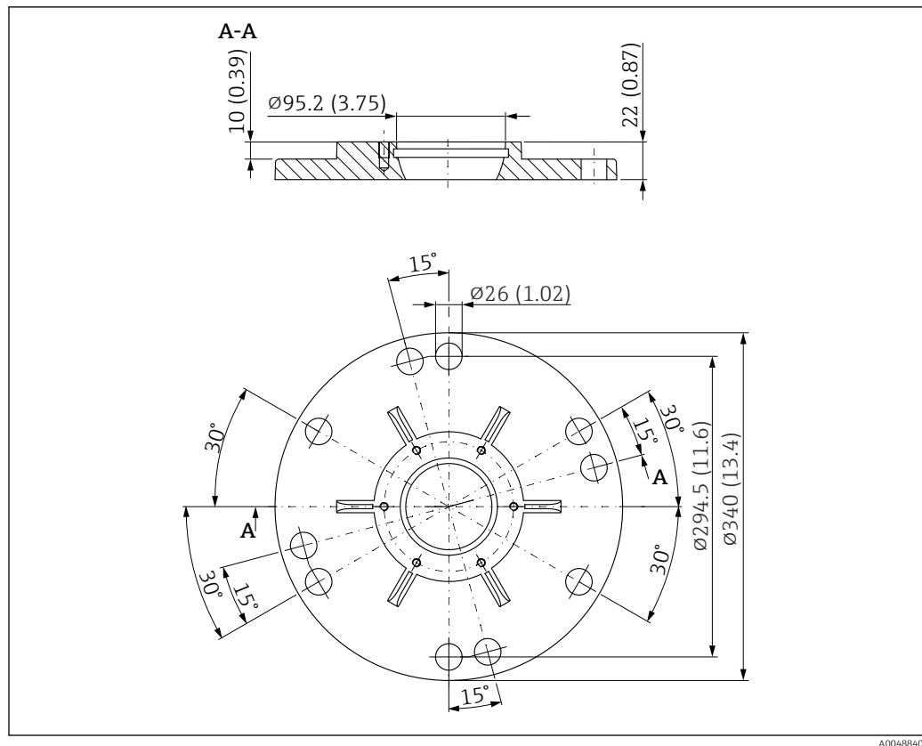
46 Dimensions of UNI flange 8"/DN200/200A for antennas with alignment unit. Unit of measurement mm (in)
