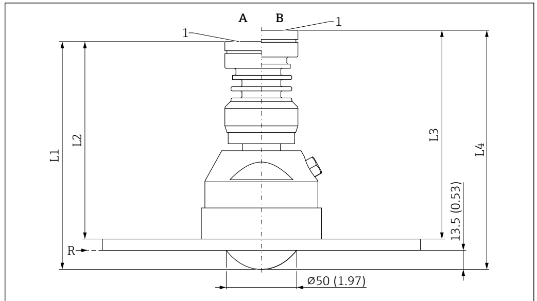
53 Dimensions of antenna flush mount, PTFE, 80 mm (3 in), with UNI flange and purge air connection. Unit of measurement mm (in)
