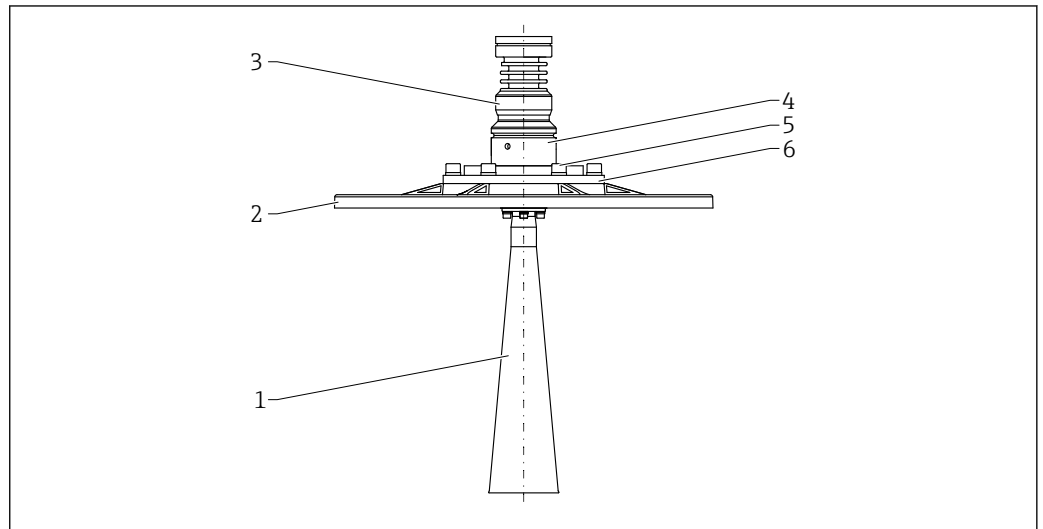
62 Material; DN65 horn antenna, with UNI flange and alignment unit. Unit of measurement mm (in)
