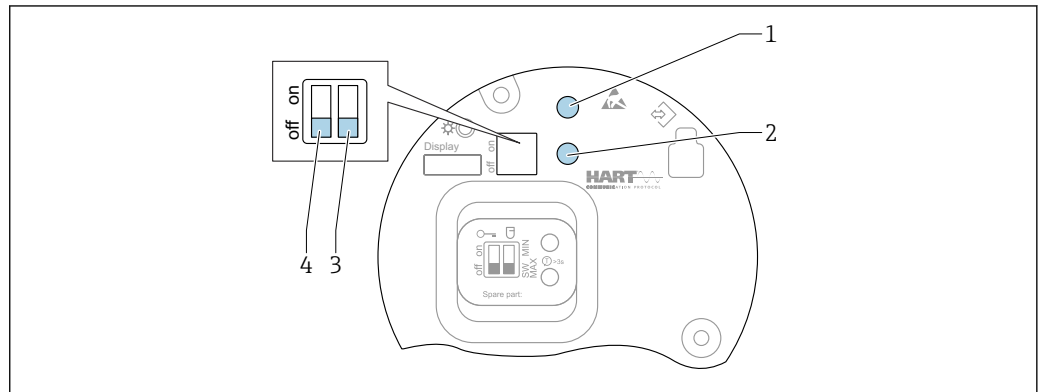
67 Operating keys and DIP switches on the HART electronic insert
