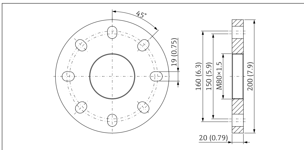
49 UNI flange 3"/DN80/80A for Drip-off antenna, PTFE, 50 mm (2 in) with purge air connection. Unit of measurement mm (in)
