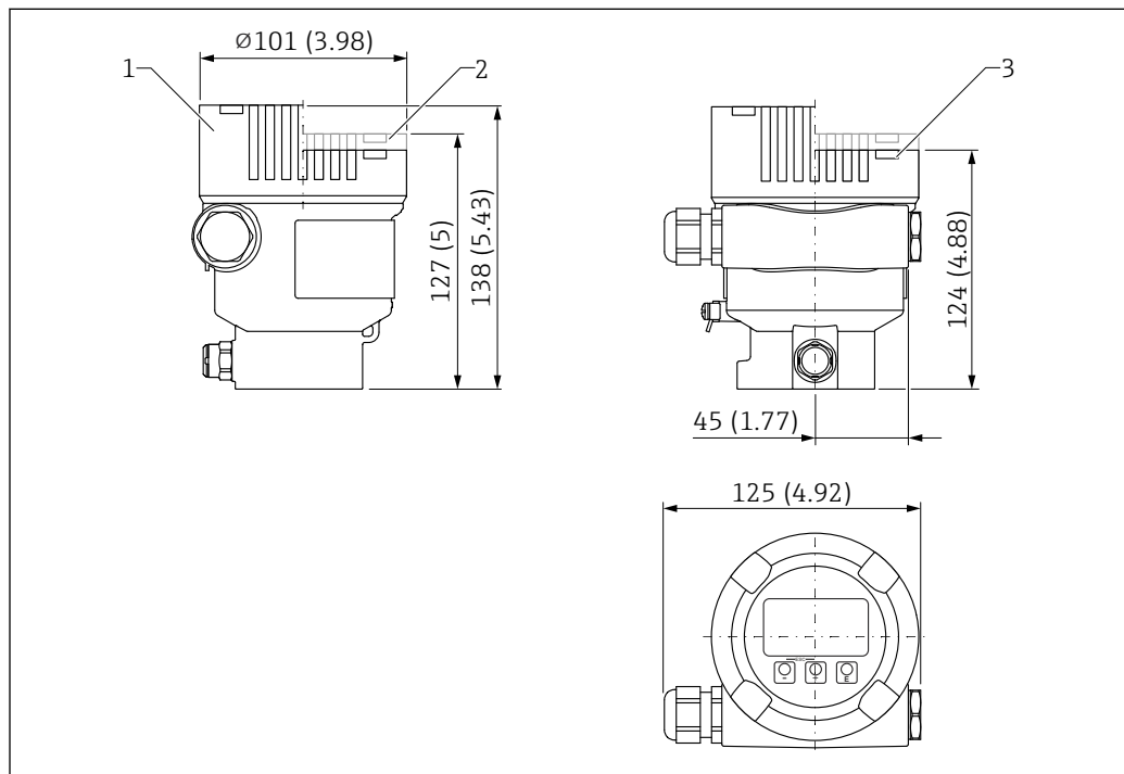
38 Dimensions of aluminum single compartment housing. Unit of measurement mm (in)
