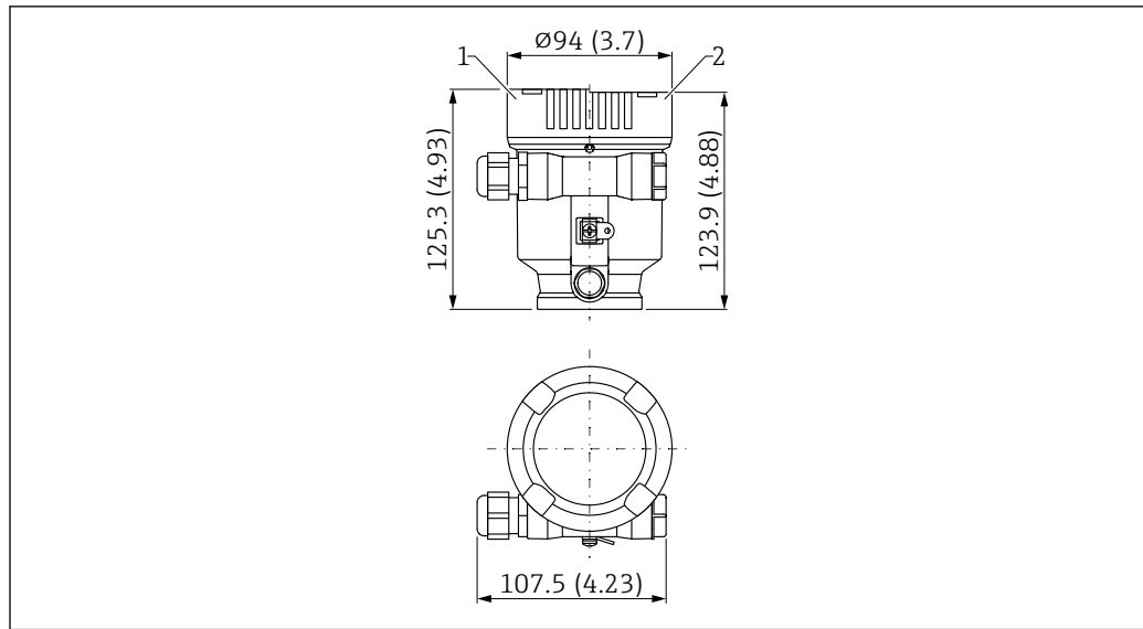
37 Dimensions of single compartment housing, plastic (PBT). Unit of measurement mm (in)
