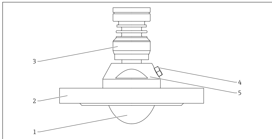
64 Material; antenna flush mount, 80 mm (3 in), with flange and purge air connection. Unit of measurement mm (in)
