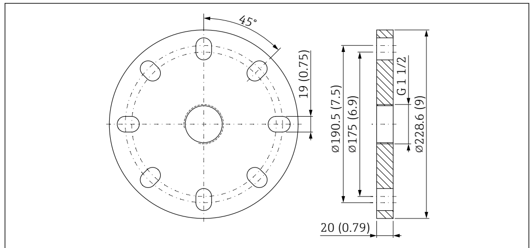
32 Dimensions of UNI flange 4"/DN100/100A. Unit of measurement mm (in)
