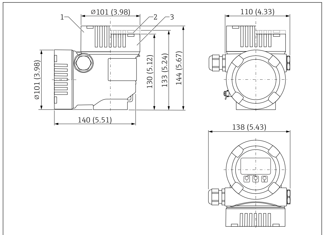
23 Dimensions of dual compartment housing, L-form. Unit of measurement mm (in)
