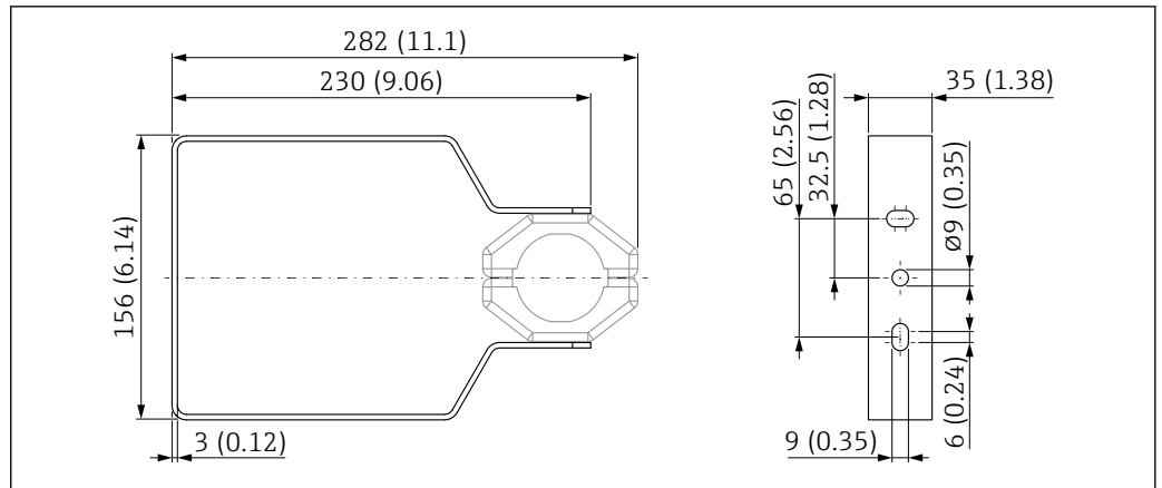
41 Dimensions of mounting bracket. Unit of measurement mm (in)
