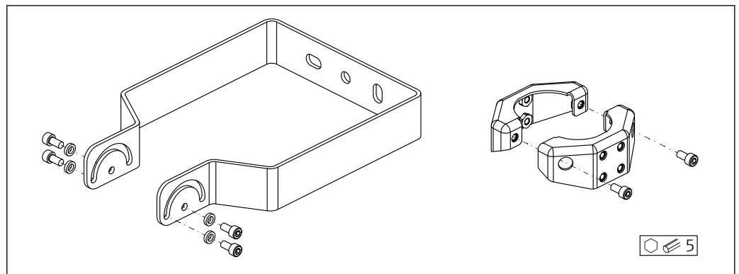
42 Scope of delivery of mounting bracket, adjustable
