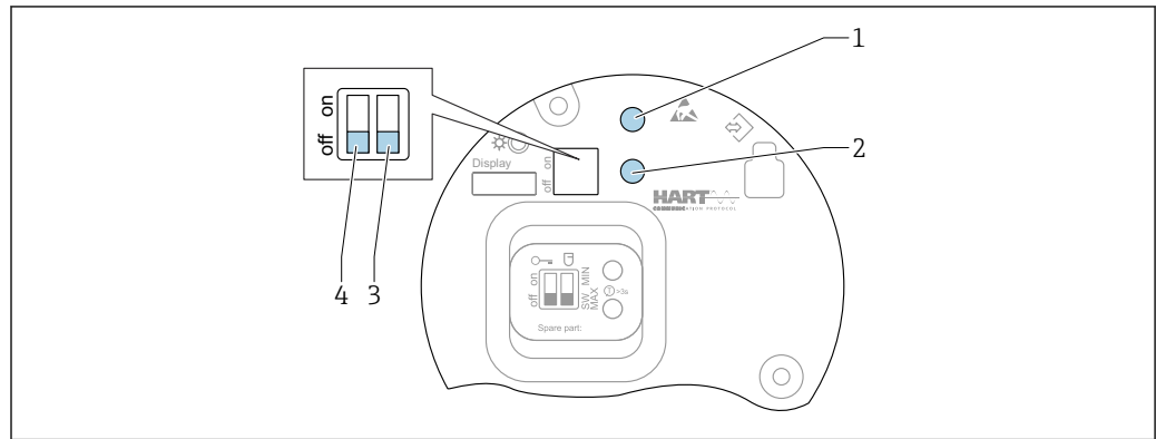
36 Operating keys and DIP switches on the HART electronic insert
